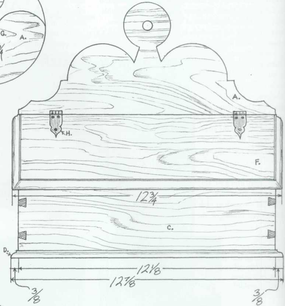
FRONT VIEW
