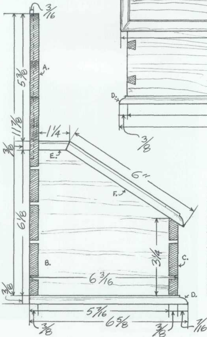
SIDE VIEW
