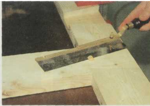
12 After the glue has dried, cut the dowels with a hand saw.
